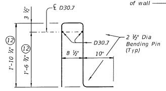
OPTIONAL WELDED WIRE REINFORCING (WWR)
