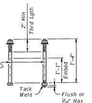
CAST-IN-PLACE ANCHOR BOLT OPTIONS
