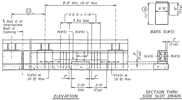
OPTIONAL SIDE SLOT DRAIN DETAILS
