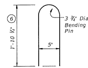
BARS wU(#5)
