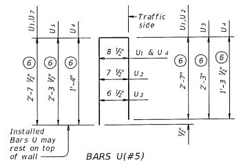
BARS U(#5)
